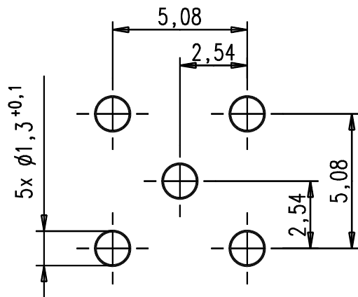
PCB - Layout
